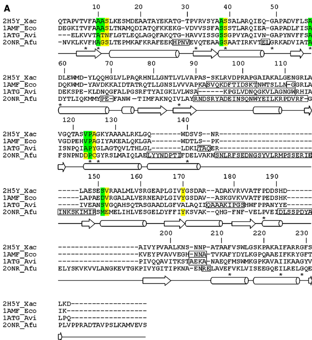
Fig. 2. The ModA binding site. (A) Amino acid structural alignment of the ModA orthologs from Xac , Eco , Avi and Afu produced with ClustalX [22] and corrected by visual inspection of the superposed structures. The numbering scheme follows the Xac ModA and the regions in boxes are structurally dissimilar from the Xac ModA structure. The asterisks underneath the sequences denote conservation, while the cylinders (helices) and arrows ( \beta -strands) indicate the secondary structures present in Xac ModA. Amino acid residues involved in molybdate interactions are shown in yellow, when forming hydrogen bonds, or in green, when possessing carbon atoms within a 3.7 Å shell. (B) Ligand-binding pocket stereo view of Xac ModA evidencing the residues that interact with molybdate. Red cylinders indicate \alpha -helices' axis and blue dashed lines indicate hydrogen bonds. The \alpha -helix close to residue Ser 12 is outside the limits of the figure. (C) Superposed ligand-binding site residues of ModA orthologs showing the equivalent residues in Xac (purple), Eco (green), Avi (blue) and Afu (yellow) proteins, respectively, that coordinate the ligand via hydrogen bonds. Residues in equivalent positions of the alignment that do not form hydrogen bonds are represented by small traces.
